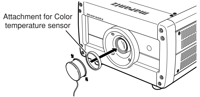
Attach the color temperature sensor so that the cable is to the bottom side of the projector as shown in the figure.
